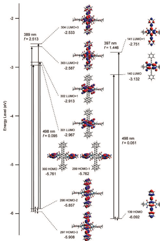
FIGURE 7. Selected frontier molecular orbitals for \mathbf{2}' (left) and \mathbf{3} (right) calculated at the B3LYP/6-311G**//B3LYP/6-31G* level of theory. Absorption wavelength and oscillator strength were calculated by TDDFT (TD/B3LYP/6-31G*).
