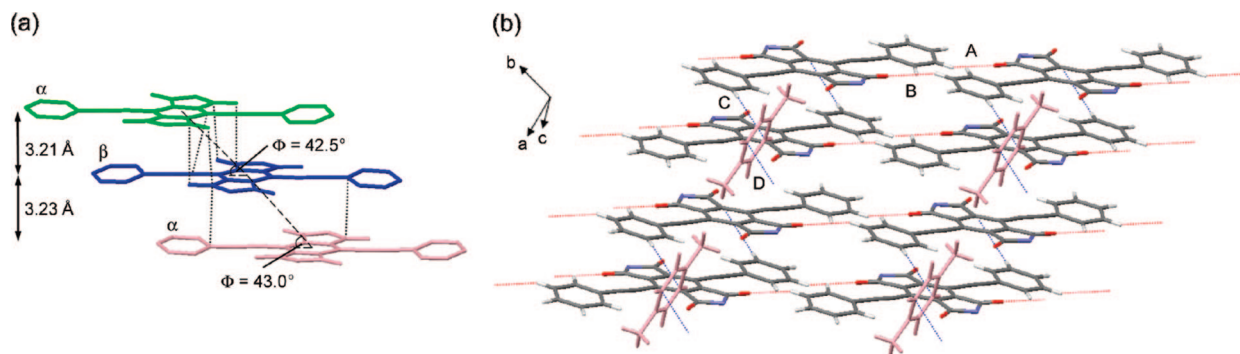
FIGURE 5. (a) Side view of the packing arrangement of (\mathbf{3})_2 \cdot p -xylene. Dotted lines show within the sum of van der Waals radius and possible electrostatic interactions. (b) Packing diagram of (\mathbf{3})_2 \cdot p -xylene. Dotted red and blue lines show C–H \cdots O and C–H \cdots \pi interactions, respectively. Butyl groups of \mathbf{3} are omitted for clarity. Selected distances (Å) of dotted lines: A, 2.47; B, 2.60; C, 2.94; D, 2.88.
