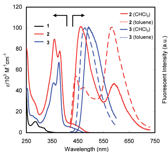
FIGURE 6. Electronic absorption of \mathbf{1} – \mathbf{3} in \text{CHCl}_3 solution and emission spectra of \mathbf{2} and \mathbf{3} .
